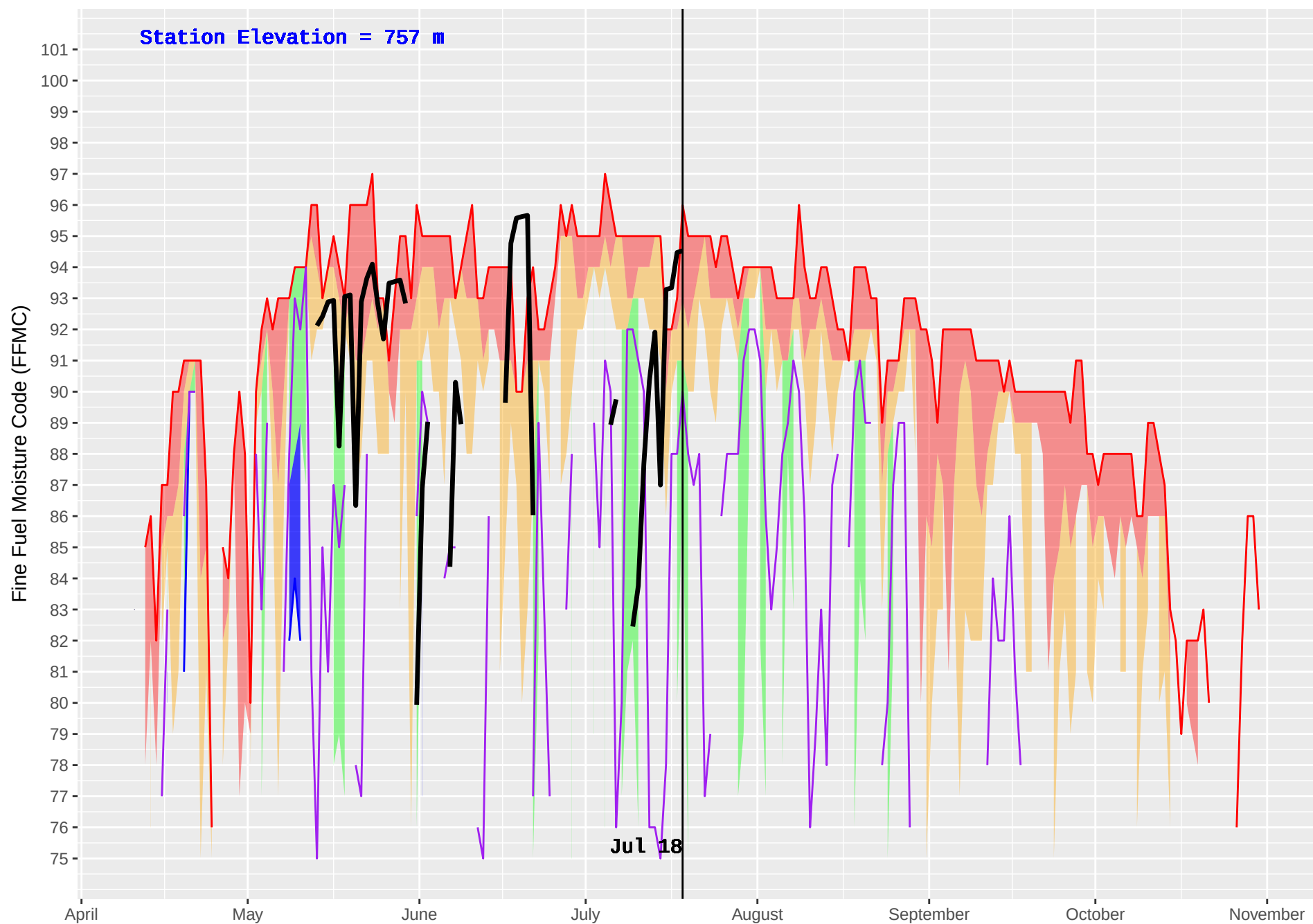
DOWNIE (905) : Historical (2005–2016) and Current (2018) Daily Fine Fuel Moisture Code (FFMC)
