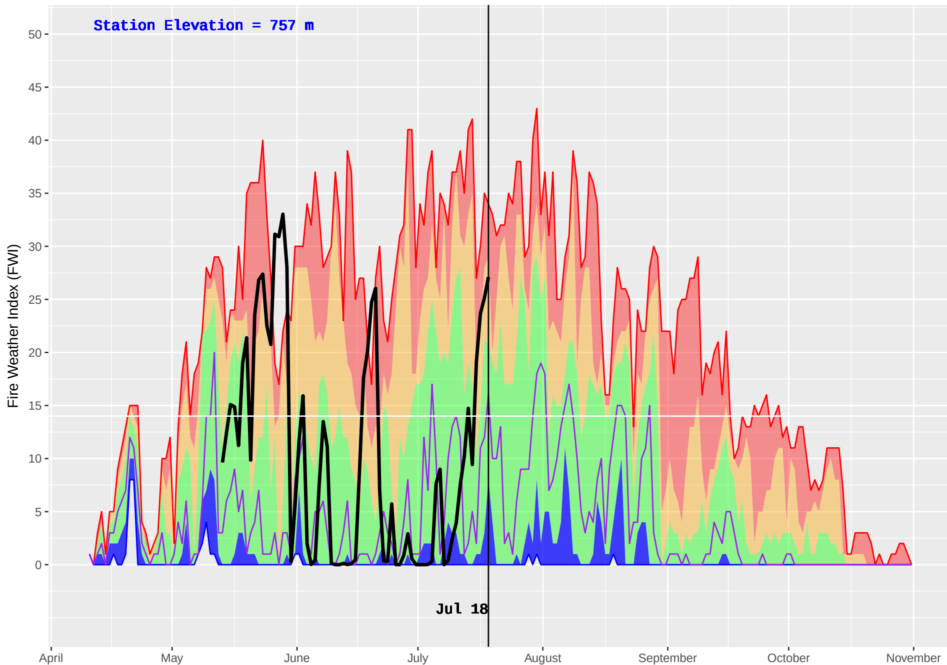
DOWNIE (905) : Historical (2005–2016) and Current (2018) Daily Fire Weather Index (FWI)
