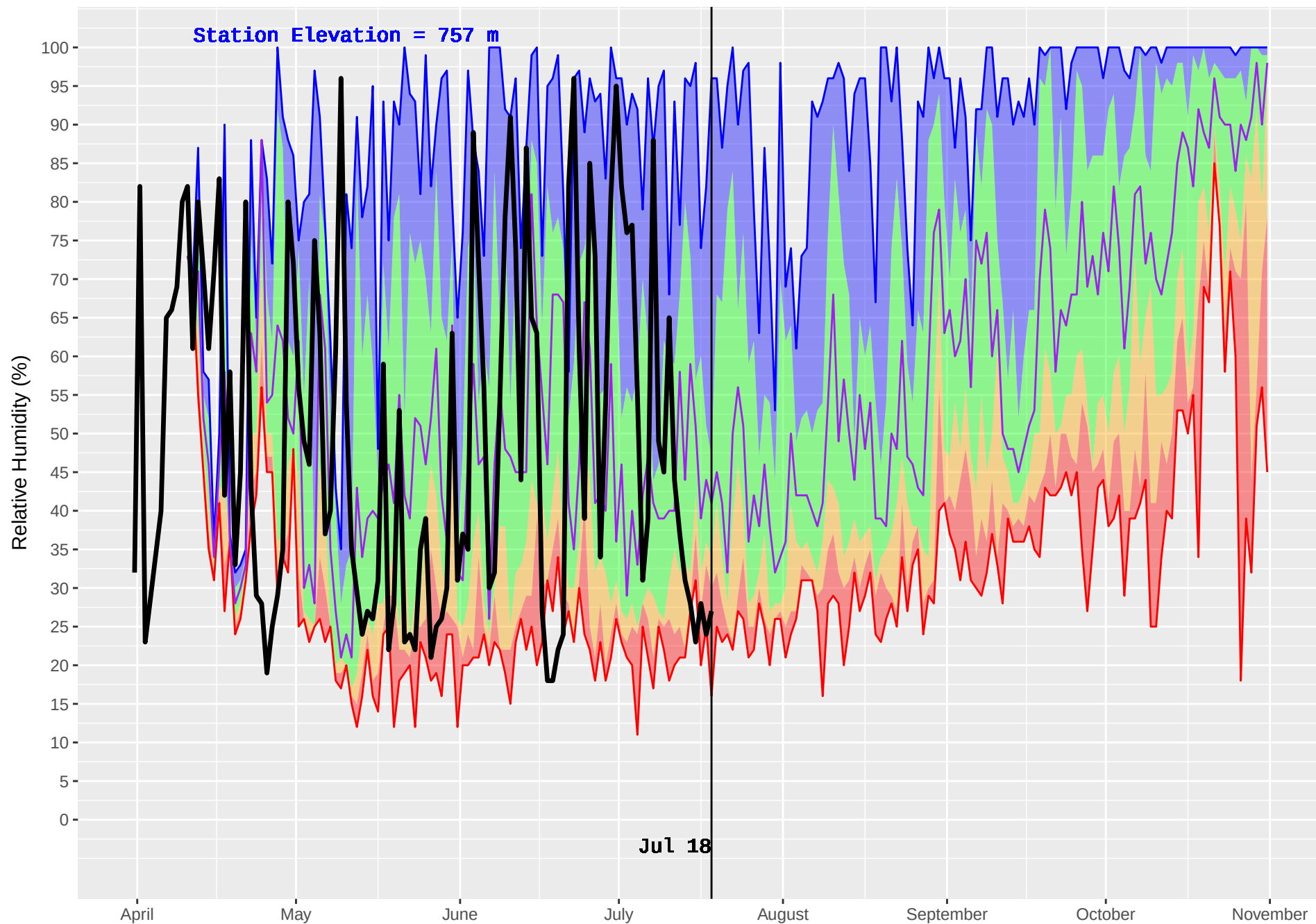
DOWNIE (905) : Historical (2005–2016) and Current (2018) Daily Relative Humidity
