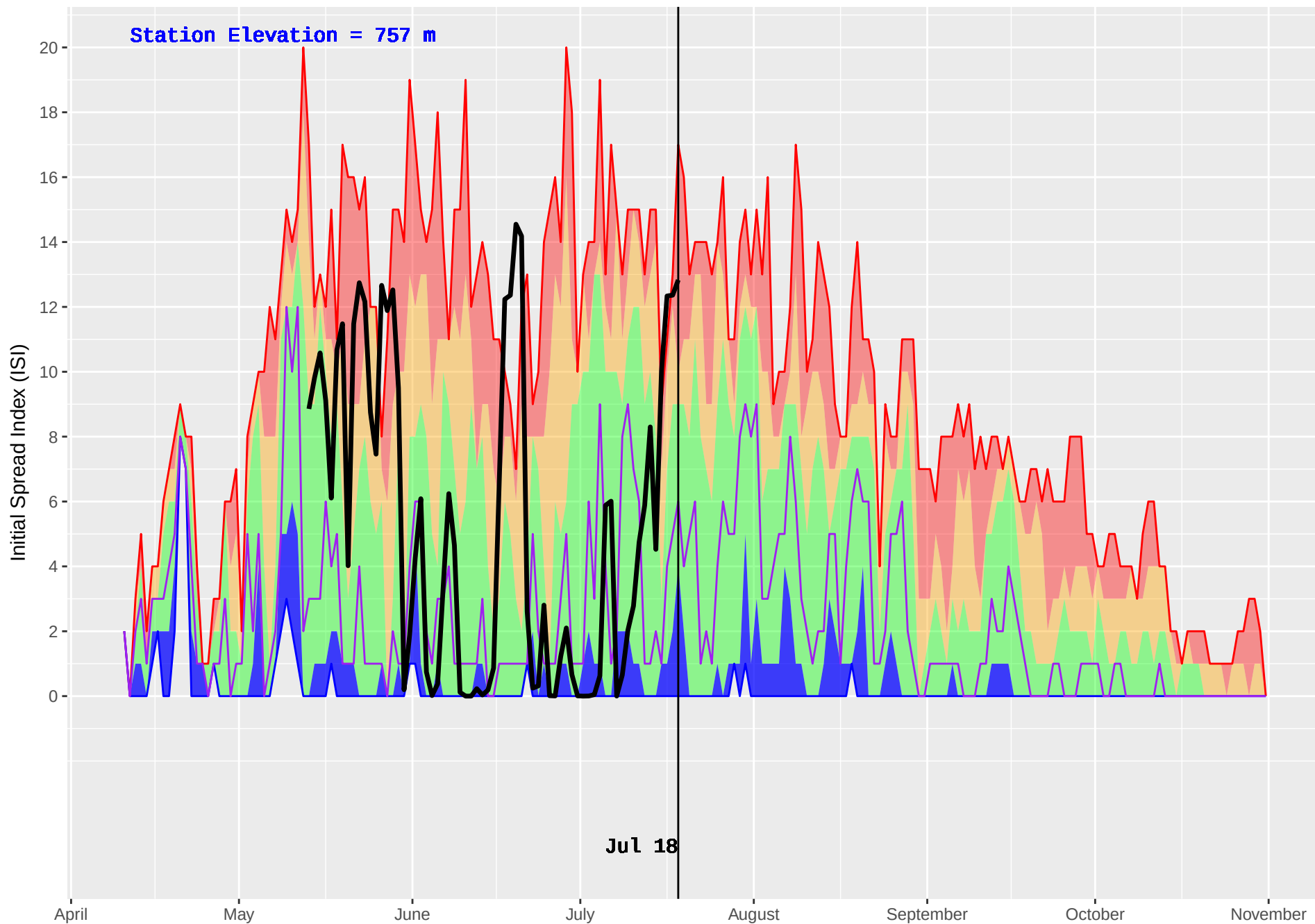
DOWNIE (905) : Historical (2005–2016) and Current (2018) Daily Initial Spread Index (ISI)
